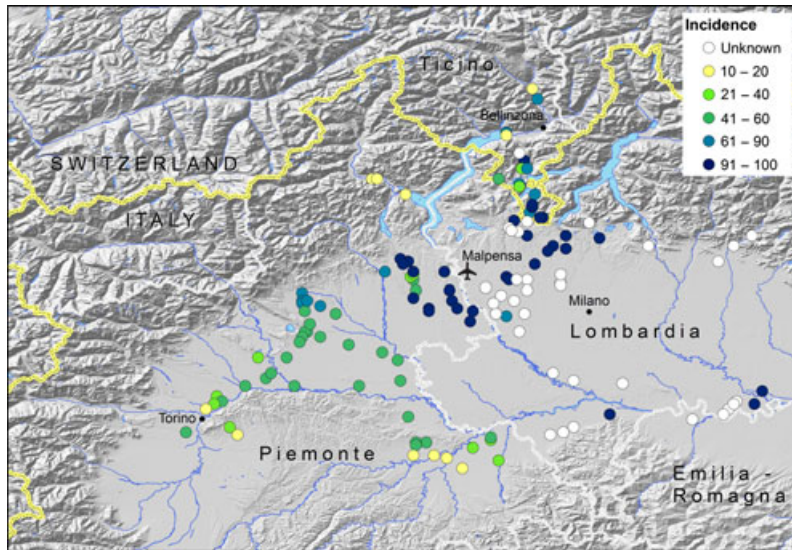
Fig. 2 Occurrence of Ophraella communa in Europe in 2013. Dots indicate sites where O. communa was found on Ambrosia artemisiifolia , colours represent the incidence of attack (% of plants attacked) at the time of observation.
